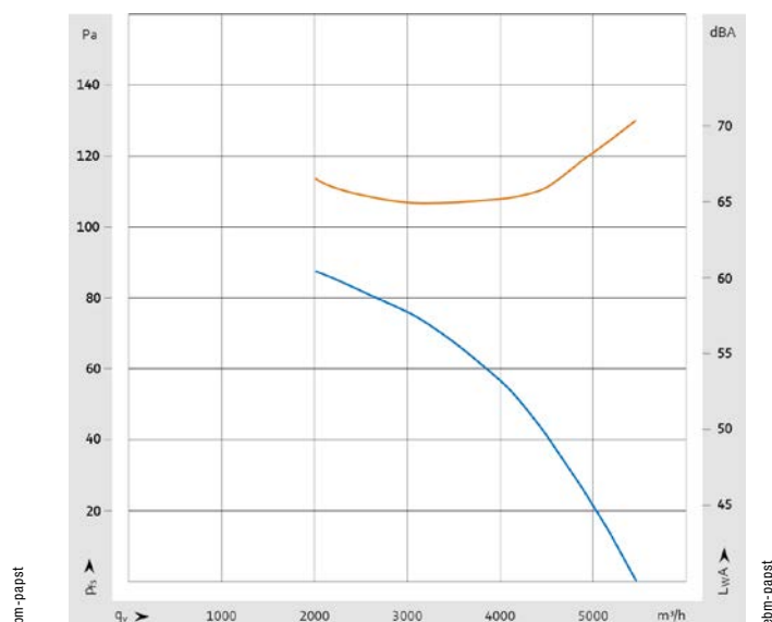
FIGURE 3: Characteristic map of the size 500 AxiEco plug-in in terms of air performance (blue characteristic curve) and noise (orange characteristic curve).
