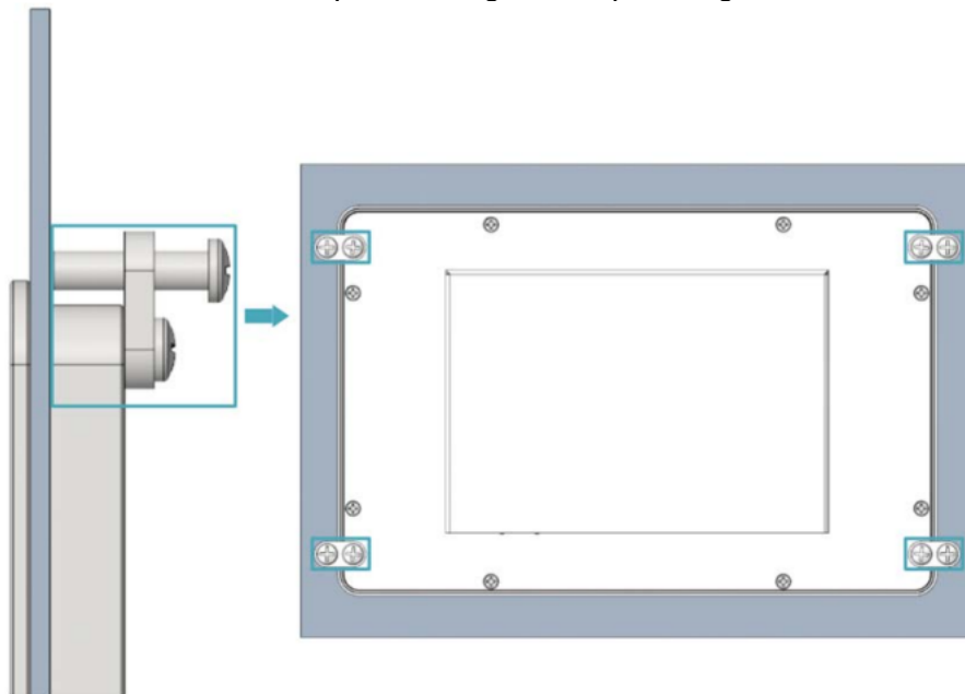
Figure 3: Panel installation.
