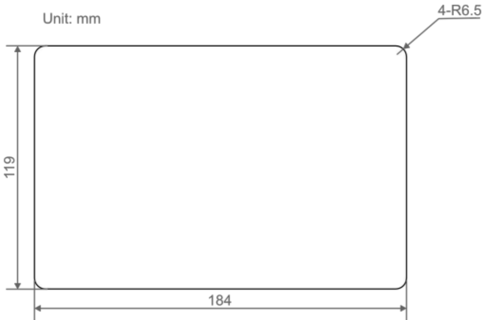
Figure 2: Cabinet hole size
