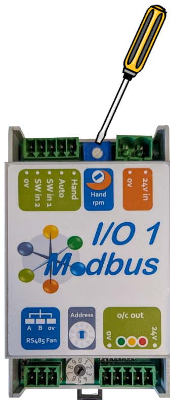
Figure 4 - Manual Hand speed adjustment
