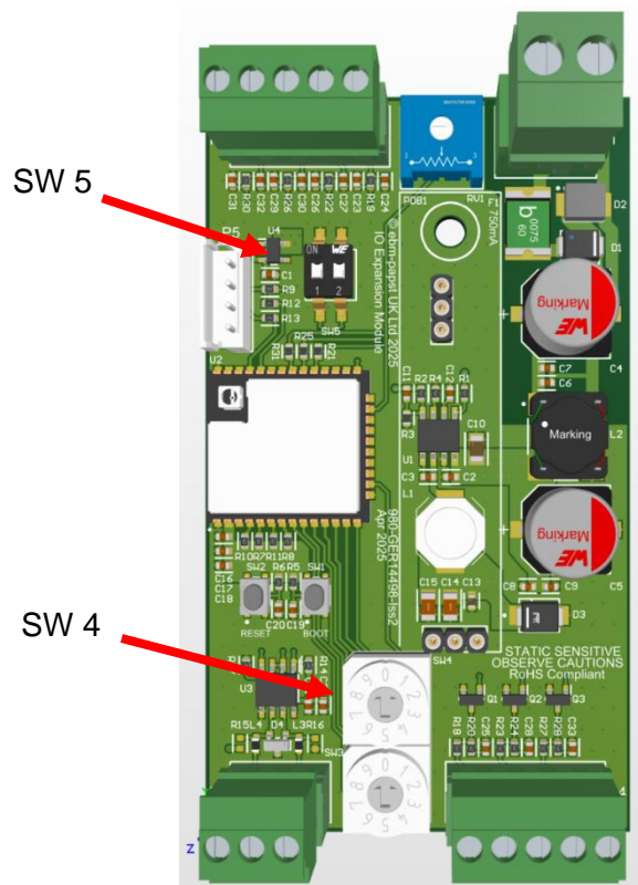
Figure 2 - Baud rate and Parity adjustment
