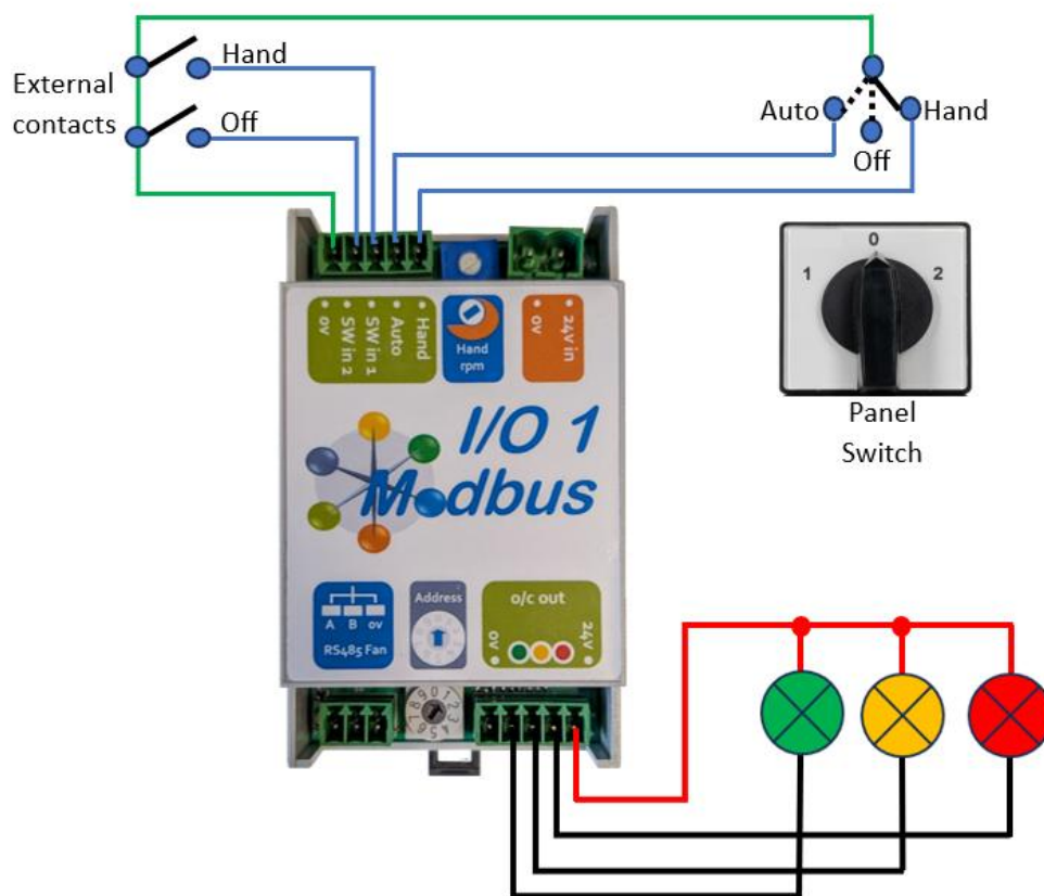
Figure 3 - Typical wiring for switches and LED's
