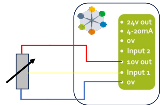
Figure 4 - Example 0-10v potentiometer input
