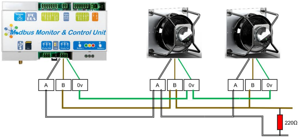
Figure 1 - RS485 connections - MMCU one end
