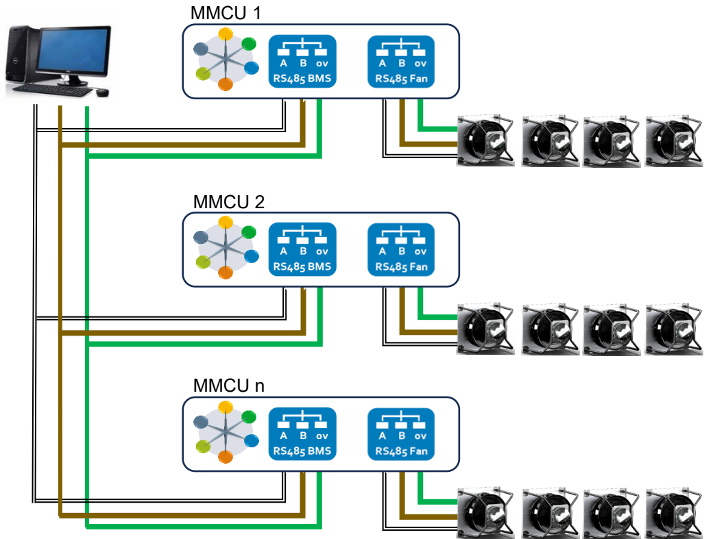
Figure 7 - Example BMS connection
